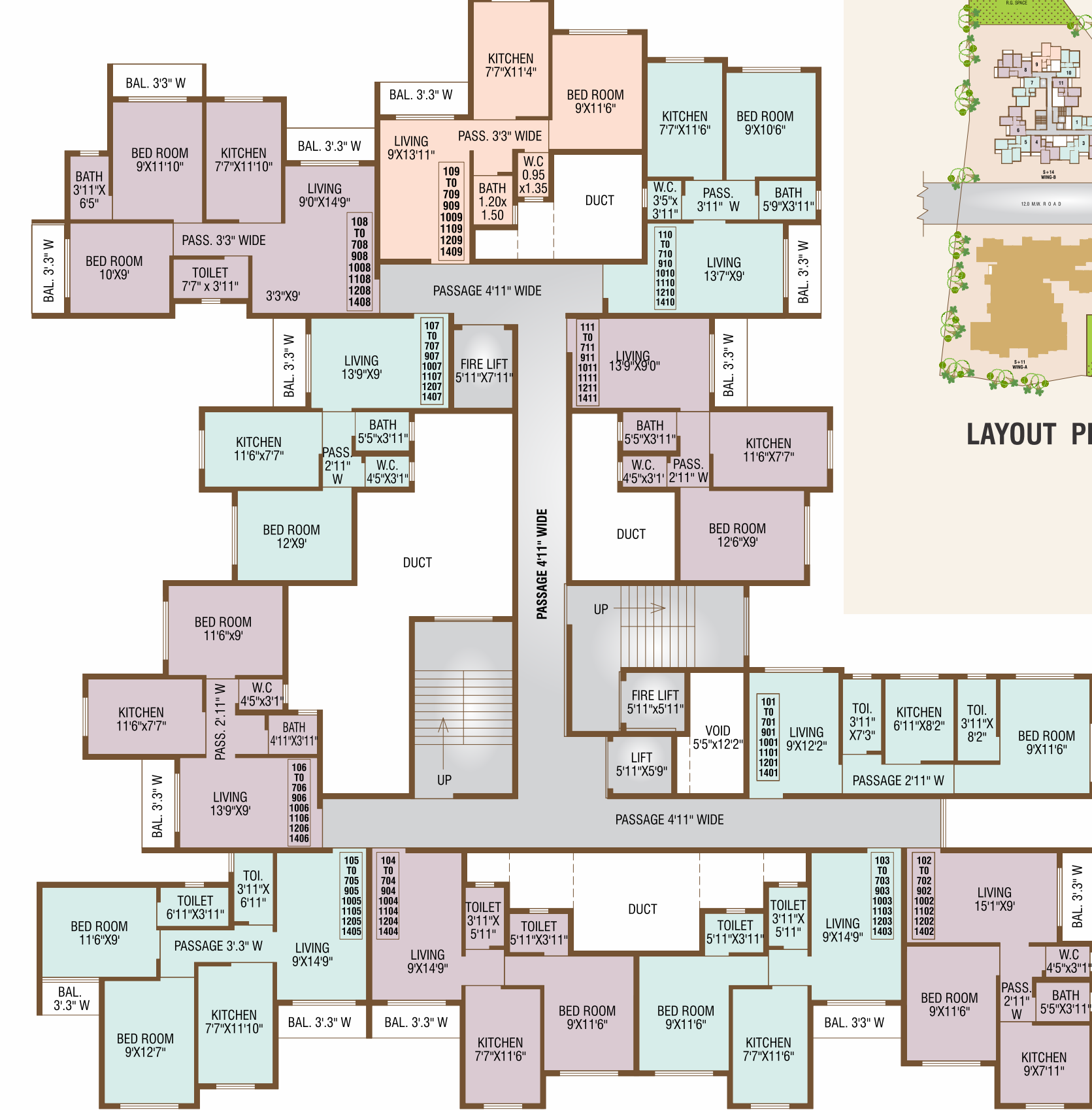
1ST,2ND,3RD,4TH,5TH,6TH,7TH,9TH,10TH, 11TH, 12TH & 14TH FLOOR (WING-B)
